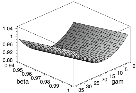
Fig. 1 The condition for convergence of the price-dividend function for the Mehra and Prescott case; the price-dividend function exists as long as, K_4 < 1 . The individual investor's discount rate, \beta = \text{beta} , is on the x -axis; his (her) coefficient of risk aversion, \gamma = \text{gam} is on the y -axis; and K_4 = K_0 e^{\frac{K_1^2 \sigma^2 - 2K_1(\phi-1)[x_0 + \sigma^2(1-\gamma)]}{2(\phi-1)^2}} is on the z -axis
